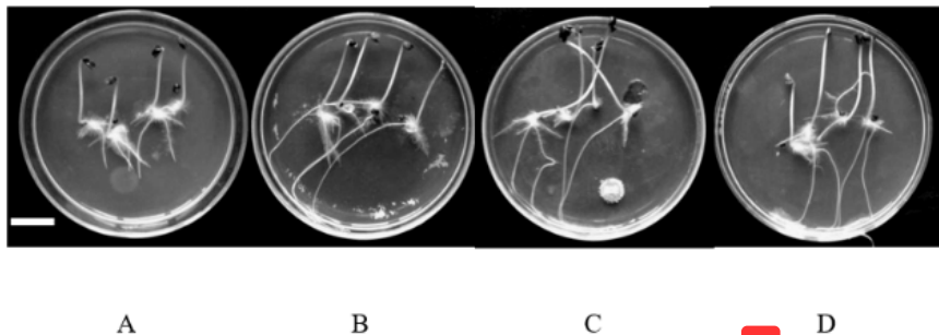
Figure 3. Early development of cauliflower ( Brassica oleracea L.) seedling. These seeds were surface sterilized and placed on water agar (5%) for germination at 25°C in a plant growth chamber for 10 days. The images showed the representative photographs of the cauliflower seedling, and each scale bar represents 2 cm
