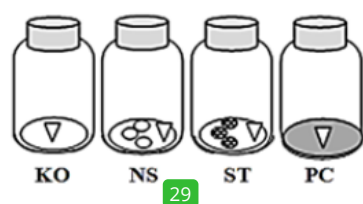
Figure 1. Schematic of in vitro evaluation of growth promoting substances produced by endophytic actinomycetes on cauliflower stalk plant growth promotion response
